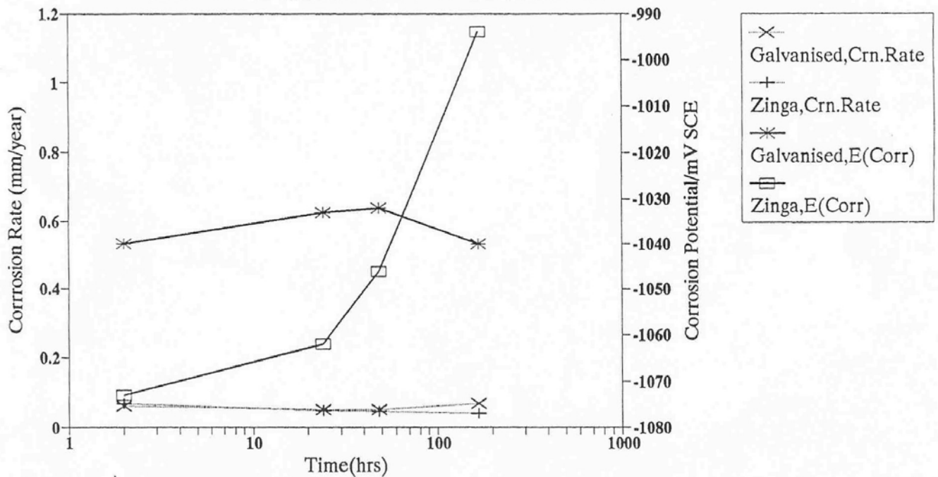
Figure 1 The variation of galvanic protection and corrosion potential with time
