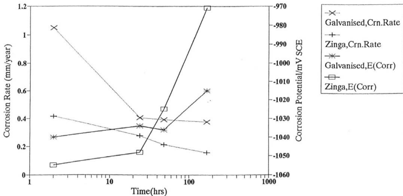
Figure 3 The variation of galvanic protection and corrosion potential with time for a protective coating to mild steel area ratio of 1:1
